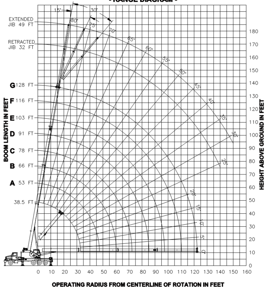
- RANGE DIAGRAM -
